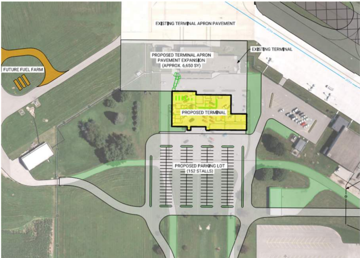
FIGURE 6 POTENTIAL SOUTH TERMINAL, PARKING, AND ACCESS ROAD
