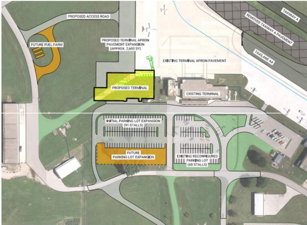
FIGURE 5 POTENTIAL WEST TERMINAL, PARKING, AND ACCESS ROAD
